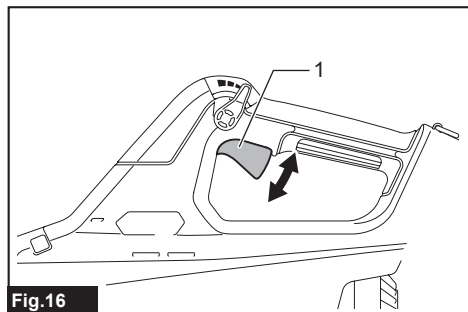
Fig.16 ► 1. Switch trigger
