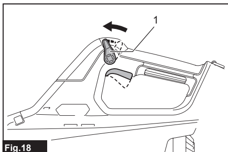
Fig.18 ► 1. Control lever
